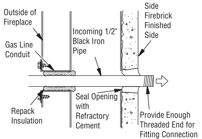
Figure 25 - Gas Line Installation
