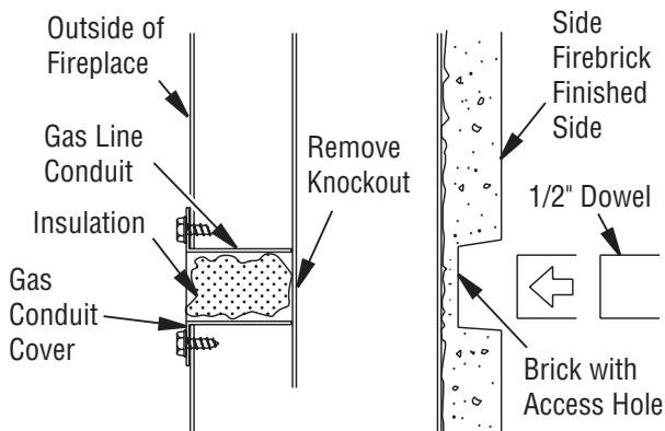
Figure 24 - Gas Line Access
