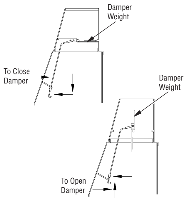
Figure 31 - Operating Damper Handle
